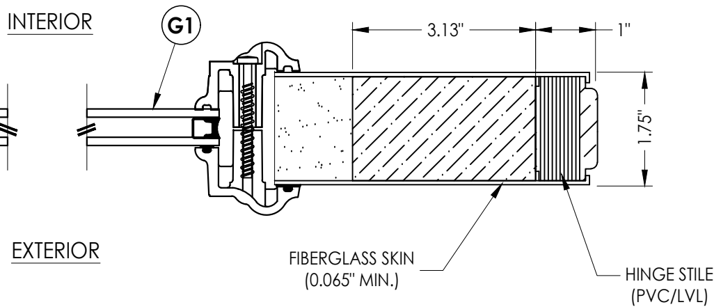
1 3 HORIZONTAL CROSS SECTION
