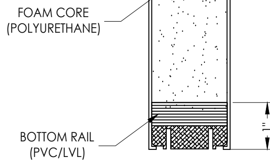
2 3 VERTICAL CROSS SECTION
